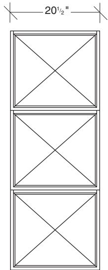
1061-49 RIGHT HANGING CABINET (one full-length door with right facing hinge)
